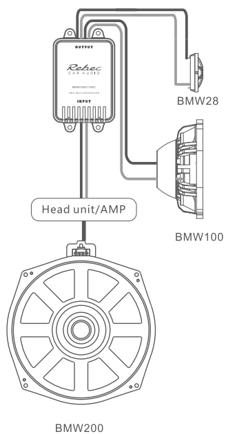
Connection diagram of BMW100C
