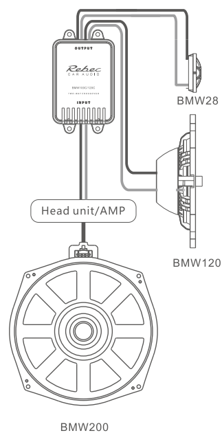
Connection diagram of BMW120C
